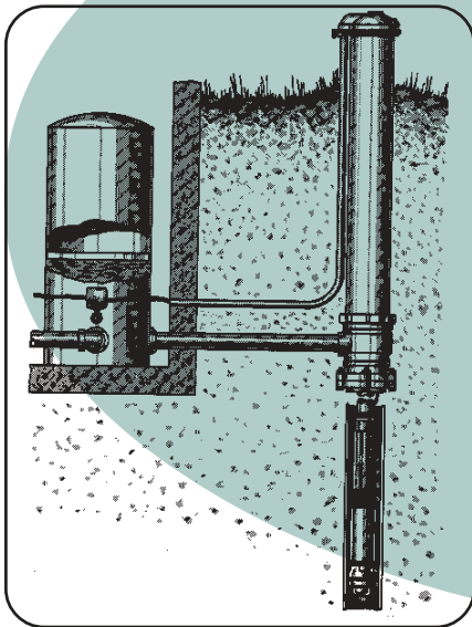
Typical general arrangement of the PS Unit with tank at the house.
